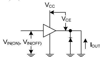
4. V_{IN(ON)} , V_{IN(OFF)}
