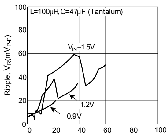
Output Current, I_{OUT} (mA)
